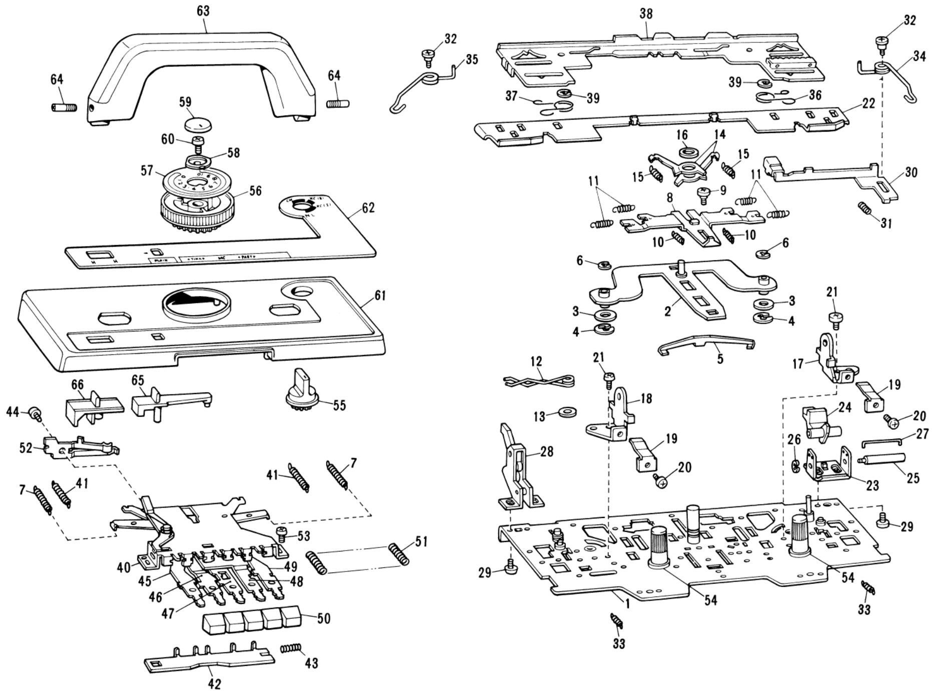
PARTS FOR CARRIAGE UPPER PART Fig: A I
