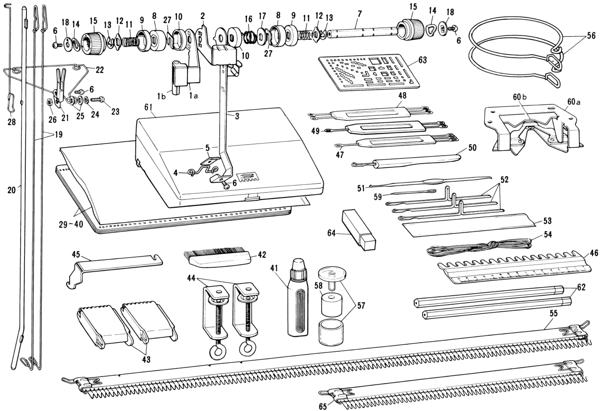
PARTS FOR ACCESSORIES
